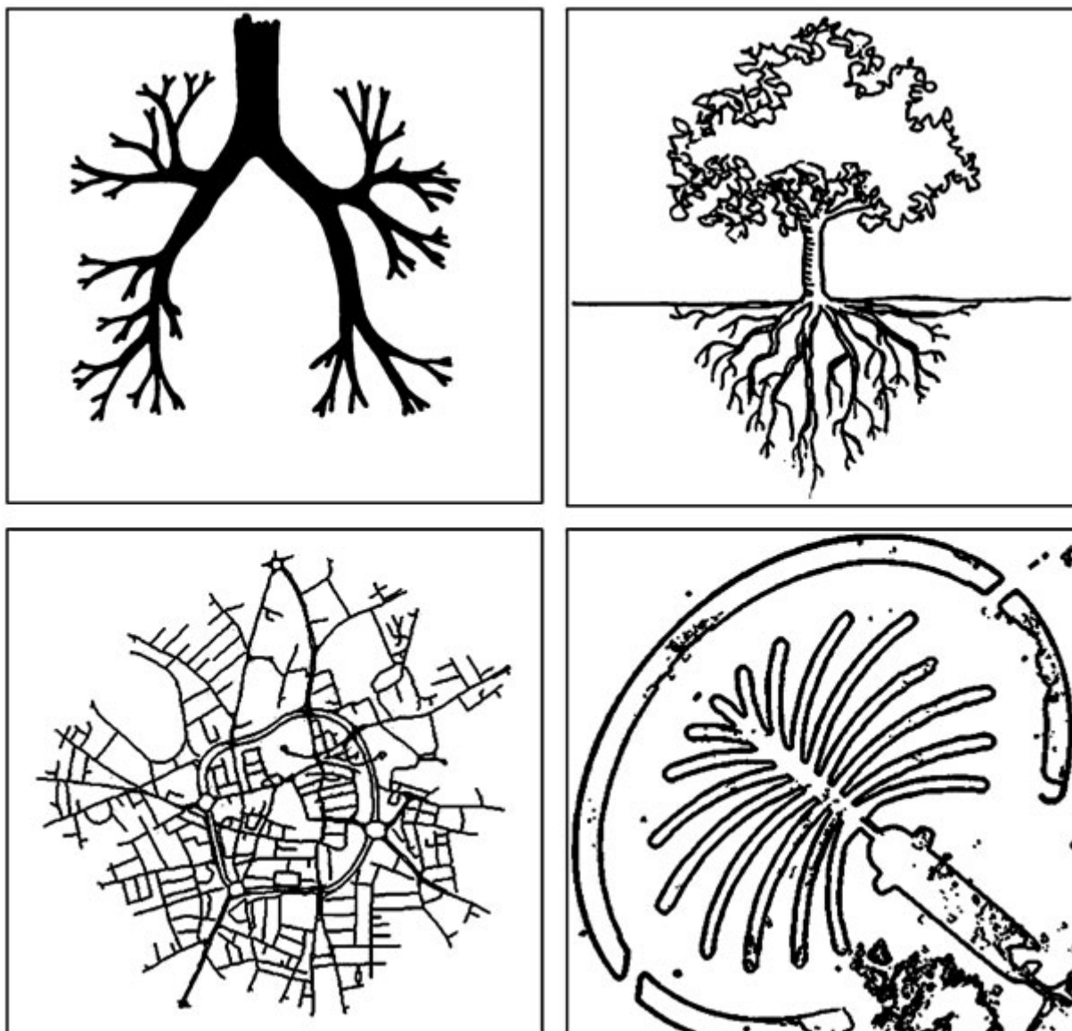
Figure 4: Space-Filling Hierarchies
